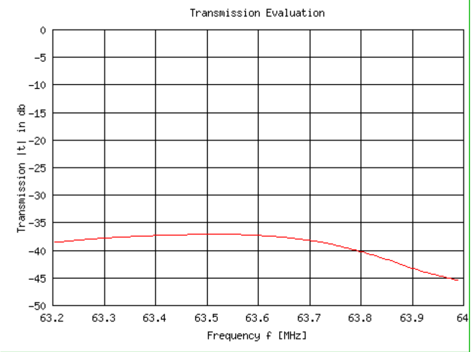
Fig. 370: BC - Transmission Evaluation
