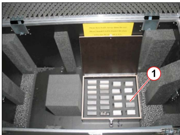
Fig. 311: Array shim device kit Pos. 1 Shim plates
