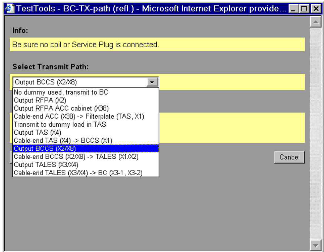
Fig. 373: Pop-up window BC-TX path (refl.) Example: Selection of TX-path termination using 50 Ohm dummies
