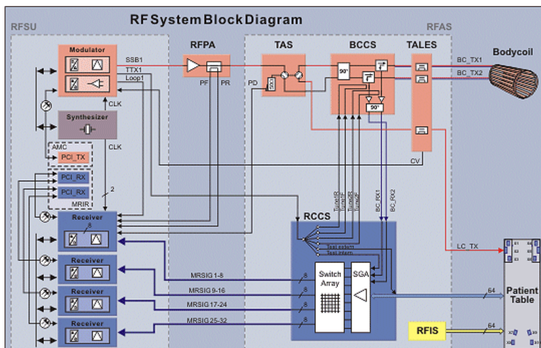
Fig. 335: RF System Block Diagram
