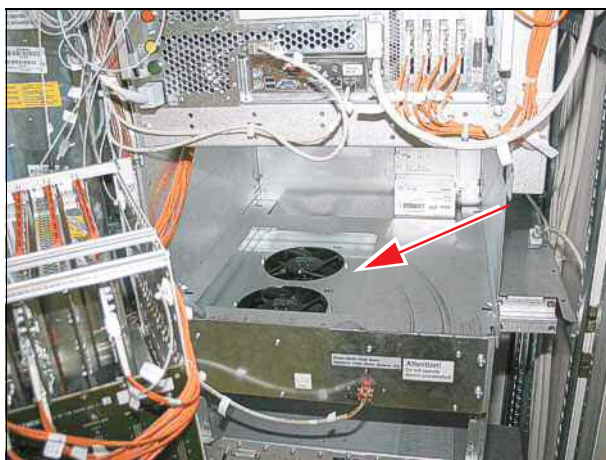
Fig. 473: Fans in ACC view
