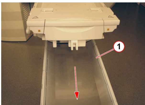
Fig. 531: Patient table support frame bottom cover
