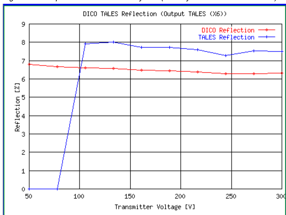
Fig. 383: Example: Transmit to Extremity Coil (Dummy connected to TALES X6)
