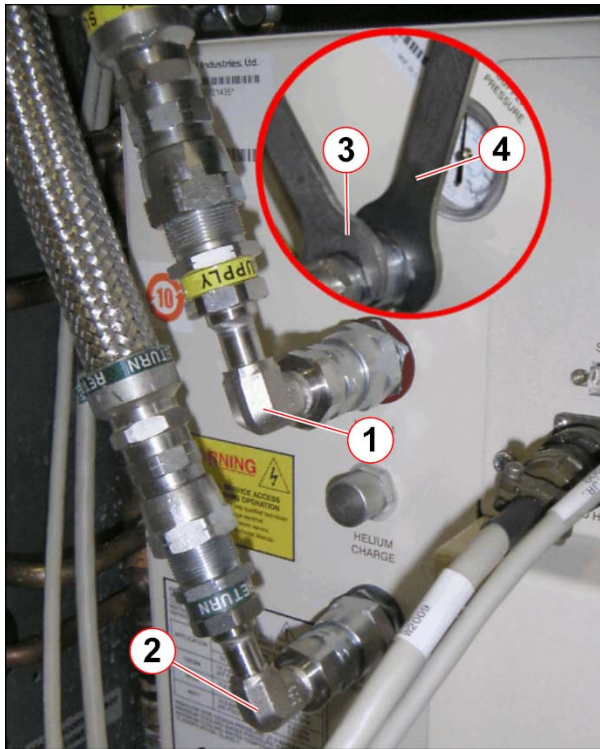
Fig. 514: F70 He compressor connections
