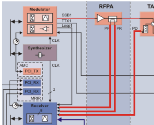
Fig. 342: RFPA Power Test
