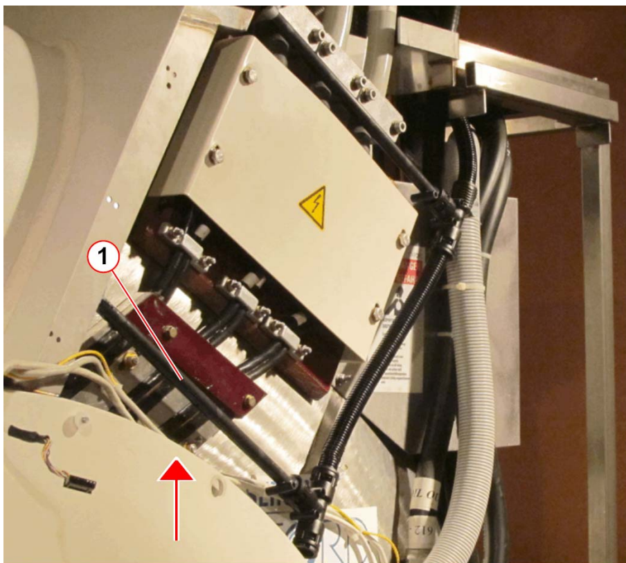
Fig. 466: Magnet service end / gradient coil connection
