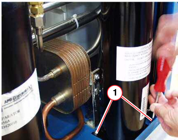
Fig. 508: Adsorber support
