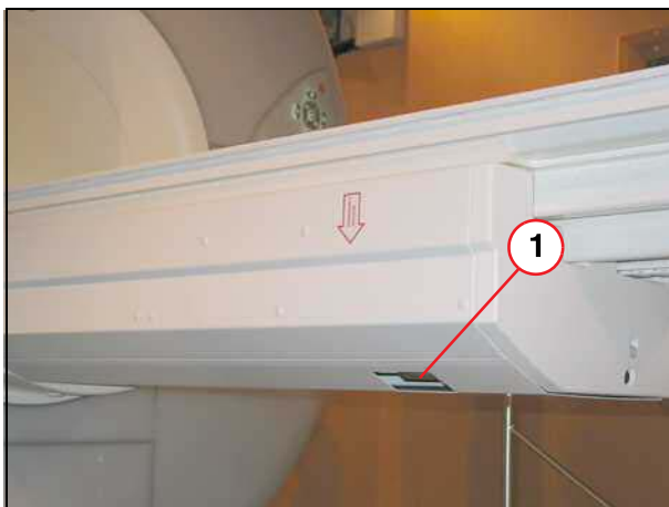
Fig. 434: Patient table Pos. 1 Emergency release
