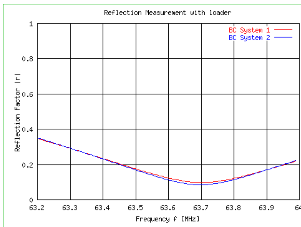
Fig. 366: BC - Reflection Evaluation
