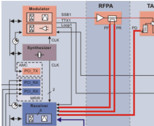
Fig. 339: RFPA Power Test
