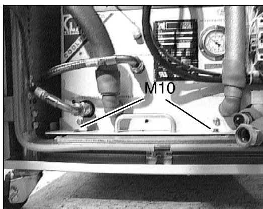
Fig. 498: Disconnection and dismantling of the cool pack
