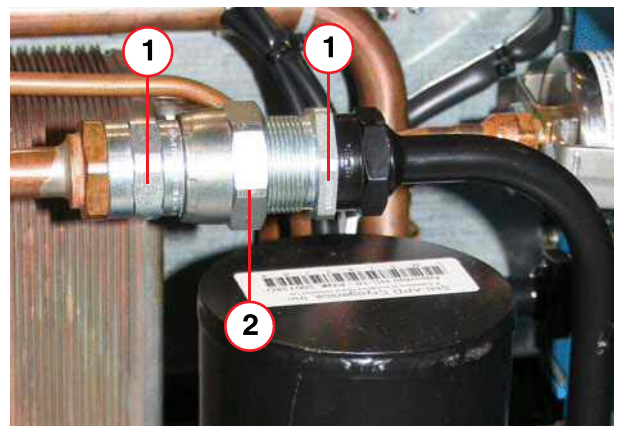
Fig. 523: F70 Adsorber - oil separator Aeroquip coupling Pos. 1 HOLD stationary nut (1" open-endspanner/ wrench) Pos. 2 TURN moveable coupling (1 3/16" open-end crow foot)
