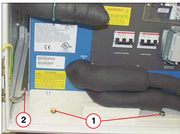
Fig. 505: Compressor attachment
