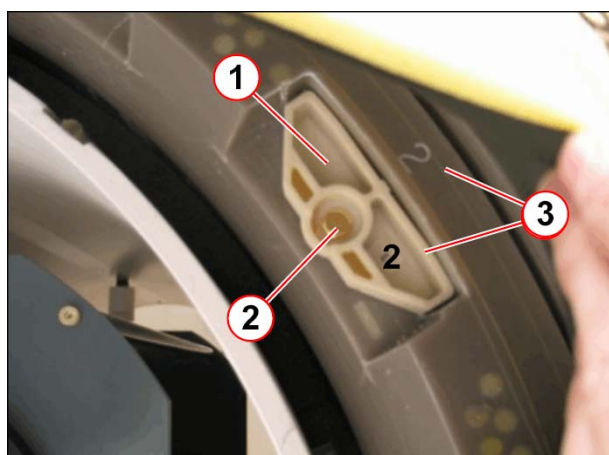
Fig. 308: Shim Tray
