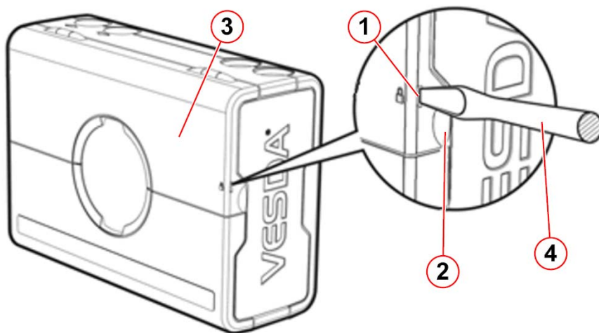
Fig. 468: Aspiration smoke detector ASD
