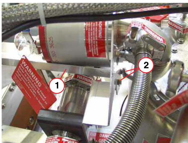
Fig. 410: Quench valve
