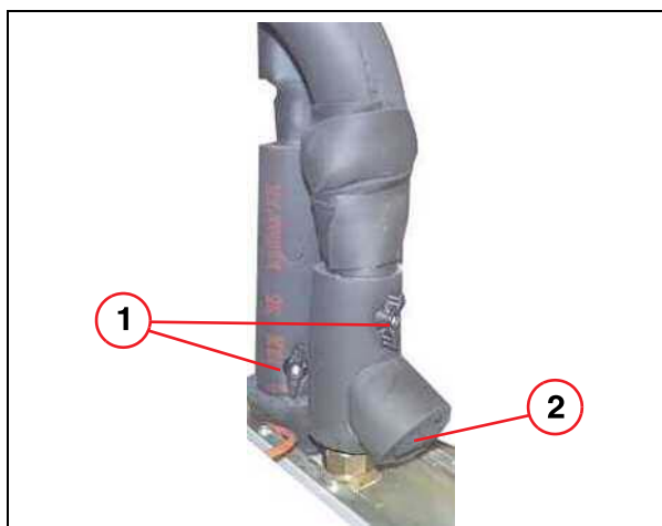
Fig. 497: Top of CCS
