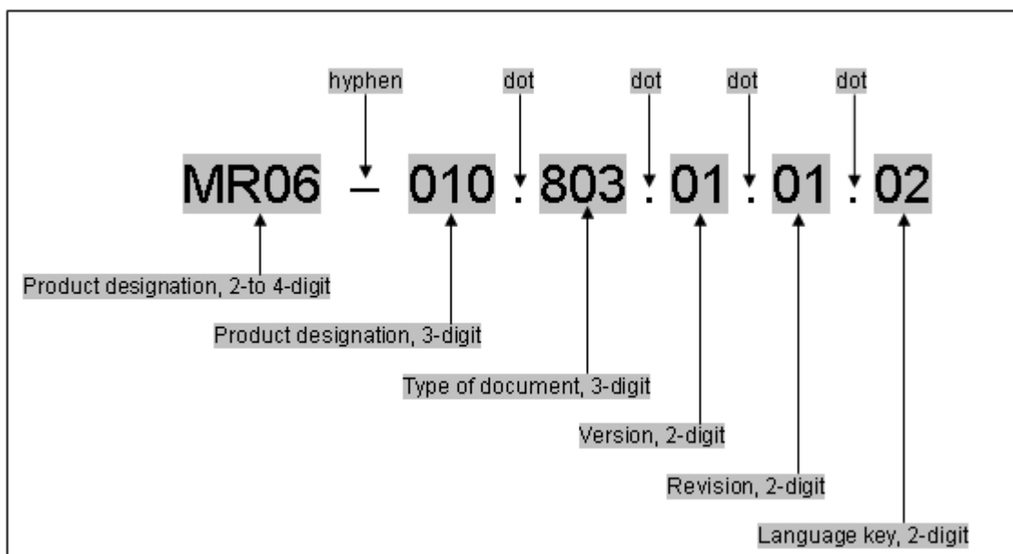
Fig. 404: Syntax print number
