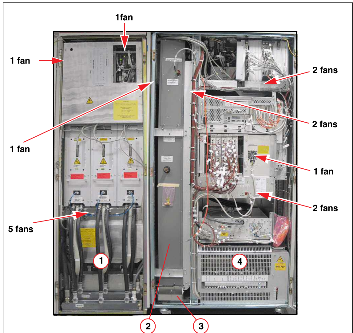
Fig. 472: GPA - CCS - ACC
