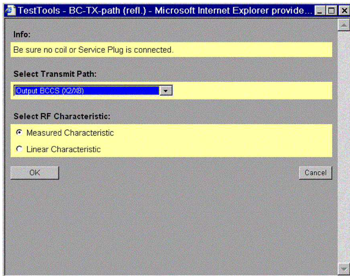
Fig. 372: Pop-up window BC-TX-path (refl.) - Selection of RF Characteristic used
