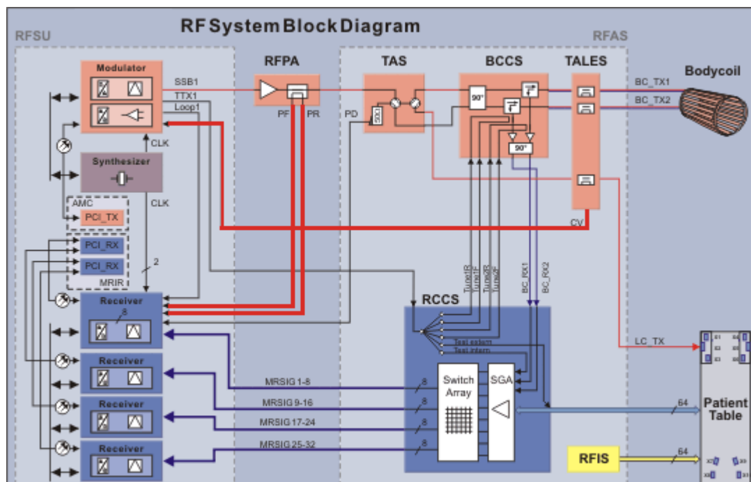
Fig. 360: BC-TX path (voltage)
