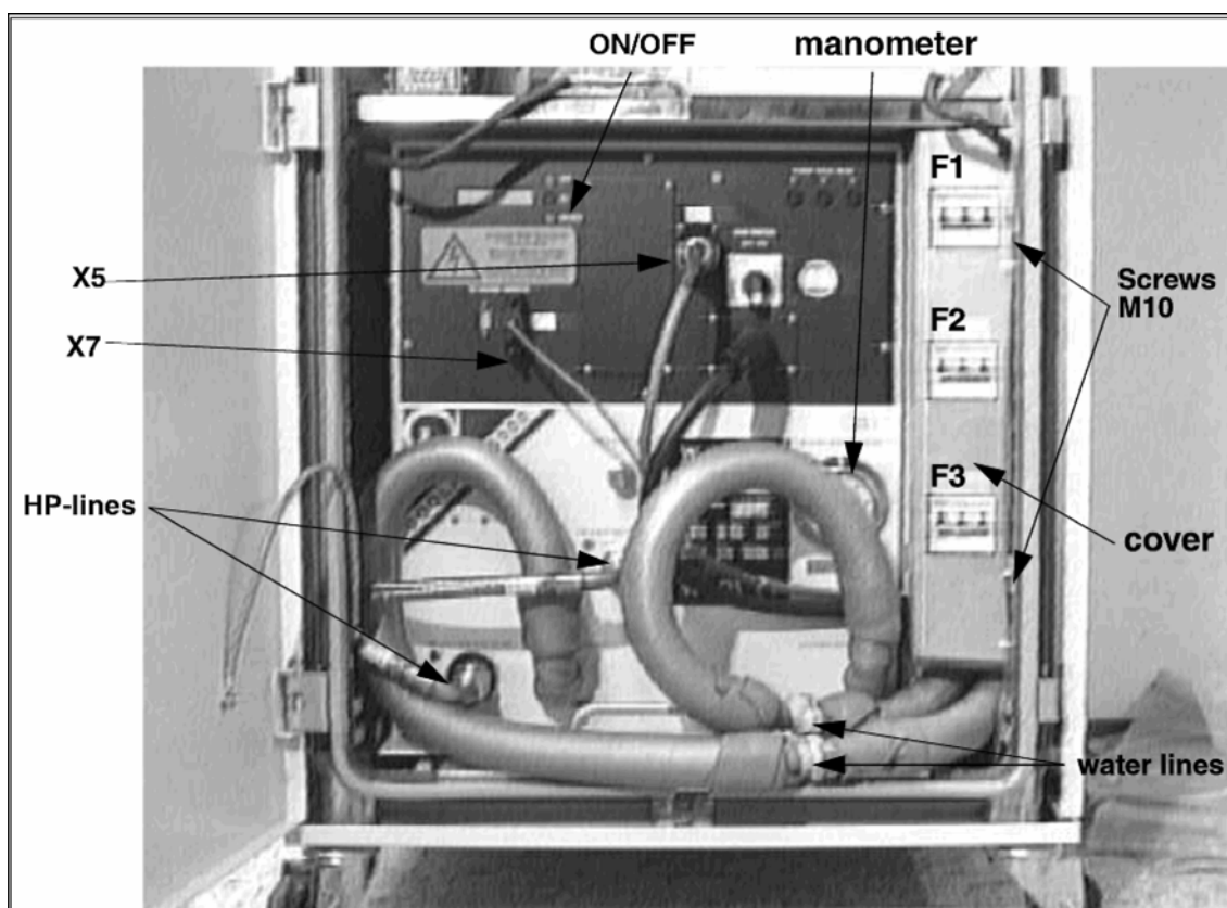
Fig. 500: Cool pack
