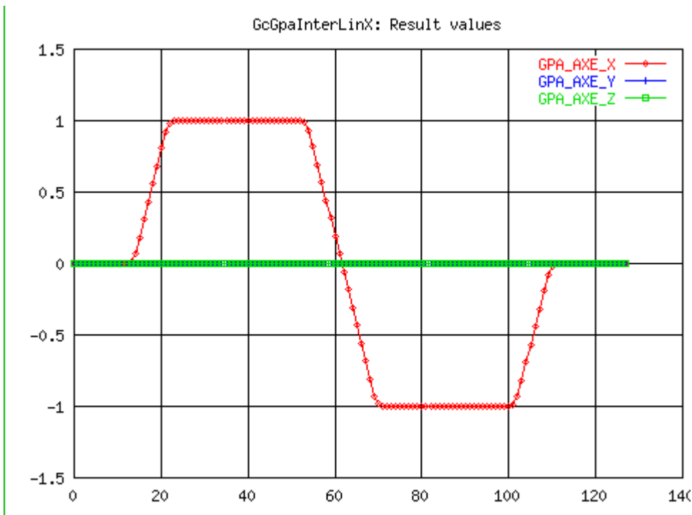
Fig. 332: Results GpaInterLin (example X axis)
