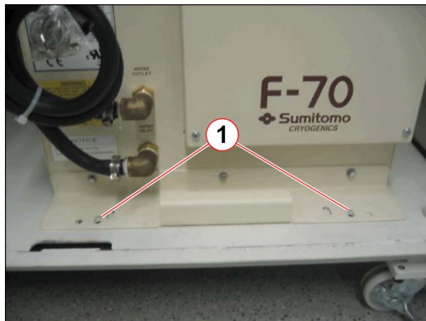
Fig. 517: F70 Compressor fixing plate
