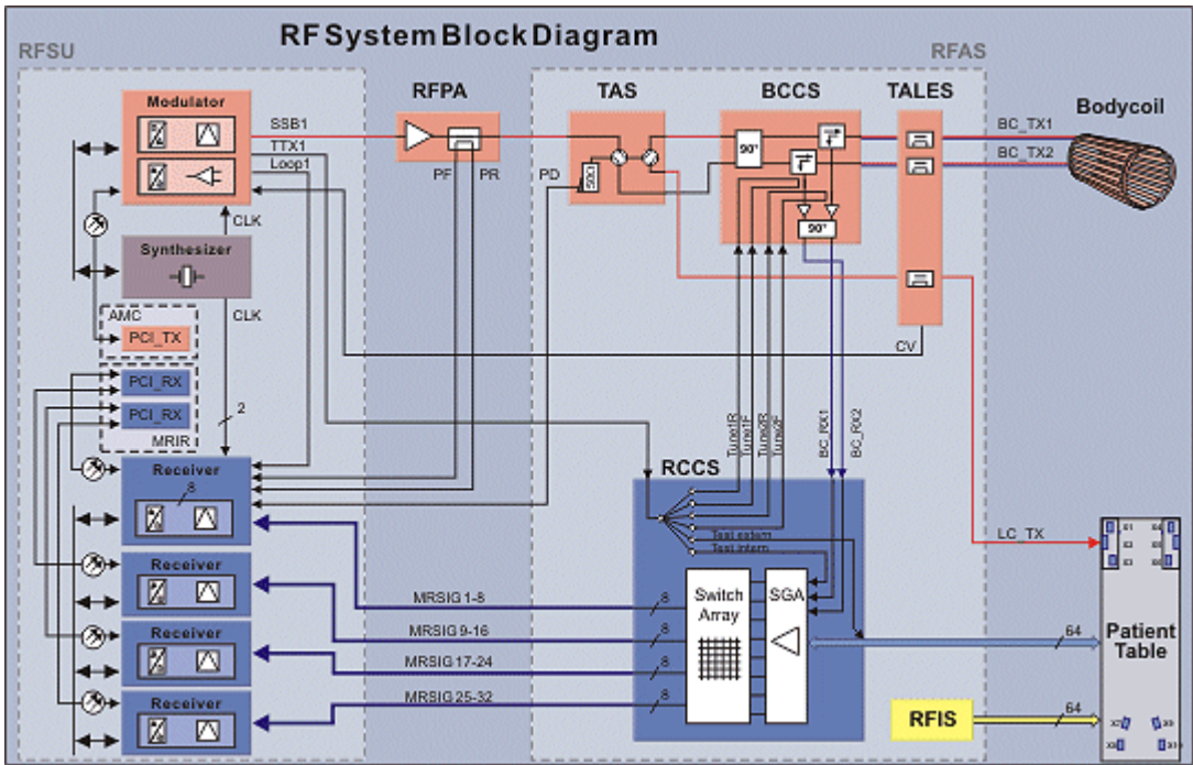
Fig. 357: BC-TX path (reflection)
