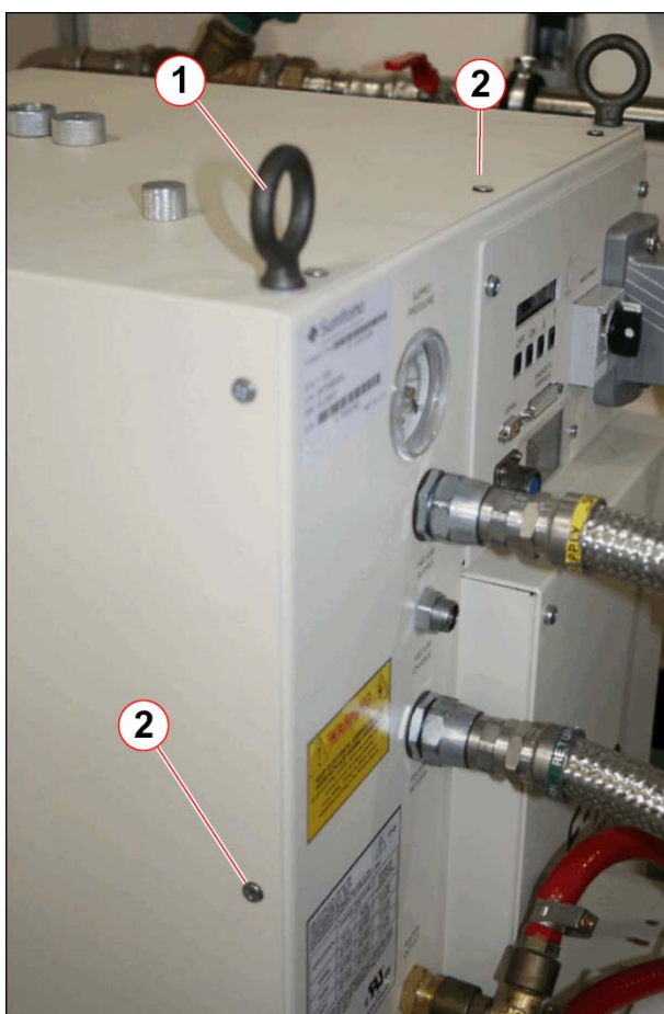
Fig. 520: F70 Lifting eyebolts and cover screws
