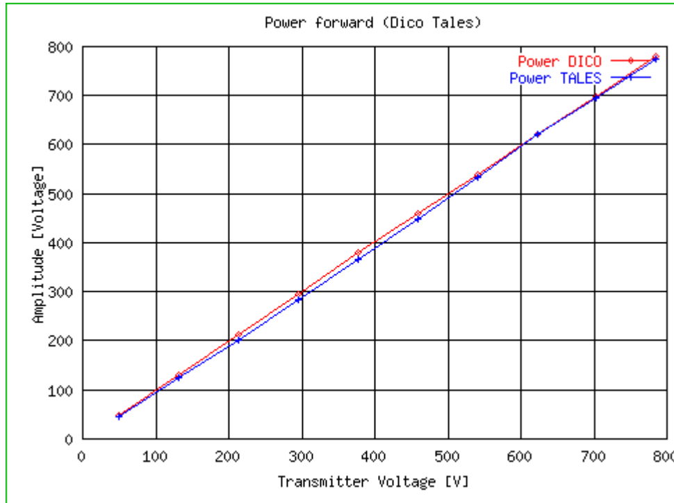
Fig. 361: Power forward measured by DICO and TALES
