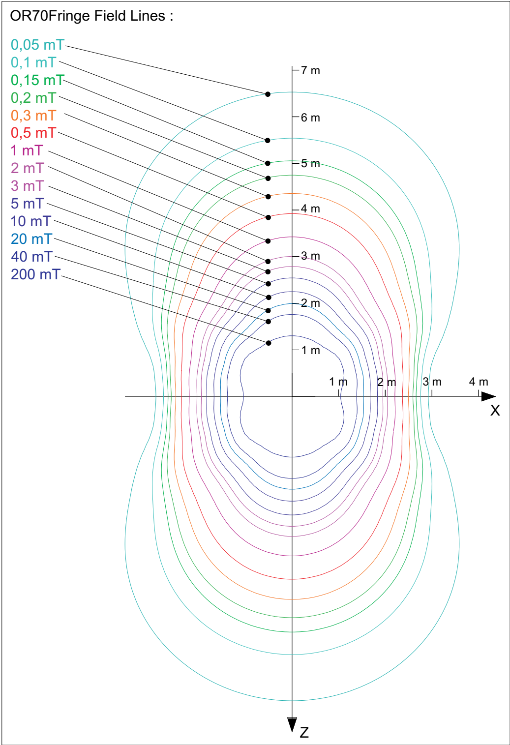
Fig. 417: Magnet fringe field
