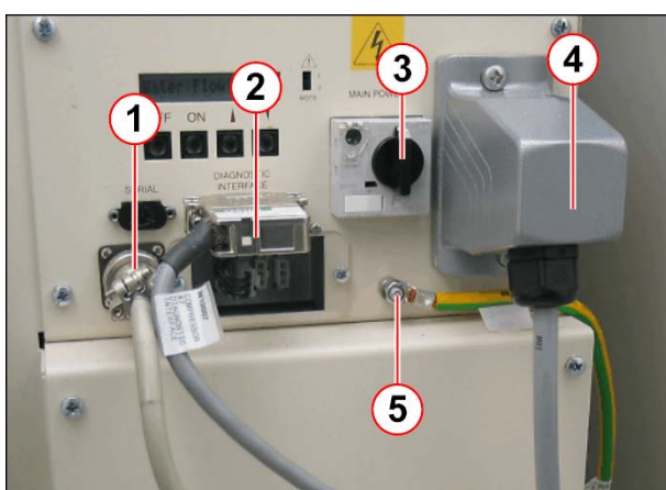
Fig. 516: F70 Electrical cable connections
