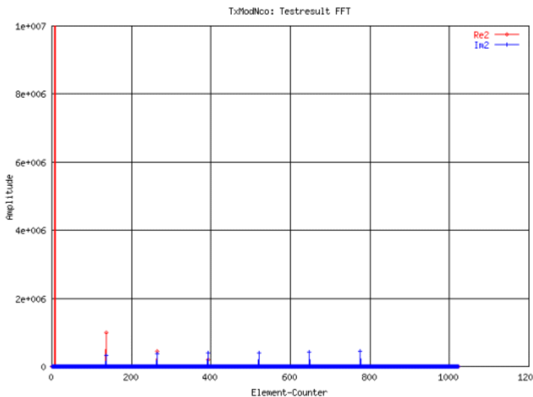
Fig. 331: FFT of the sine function
