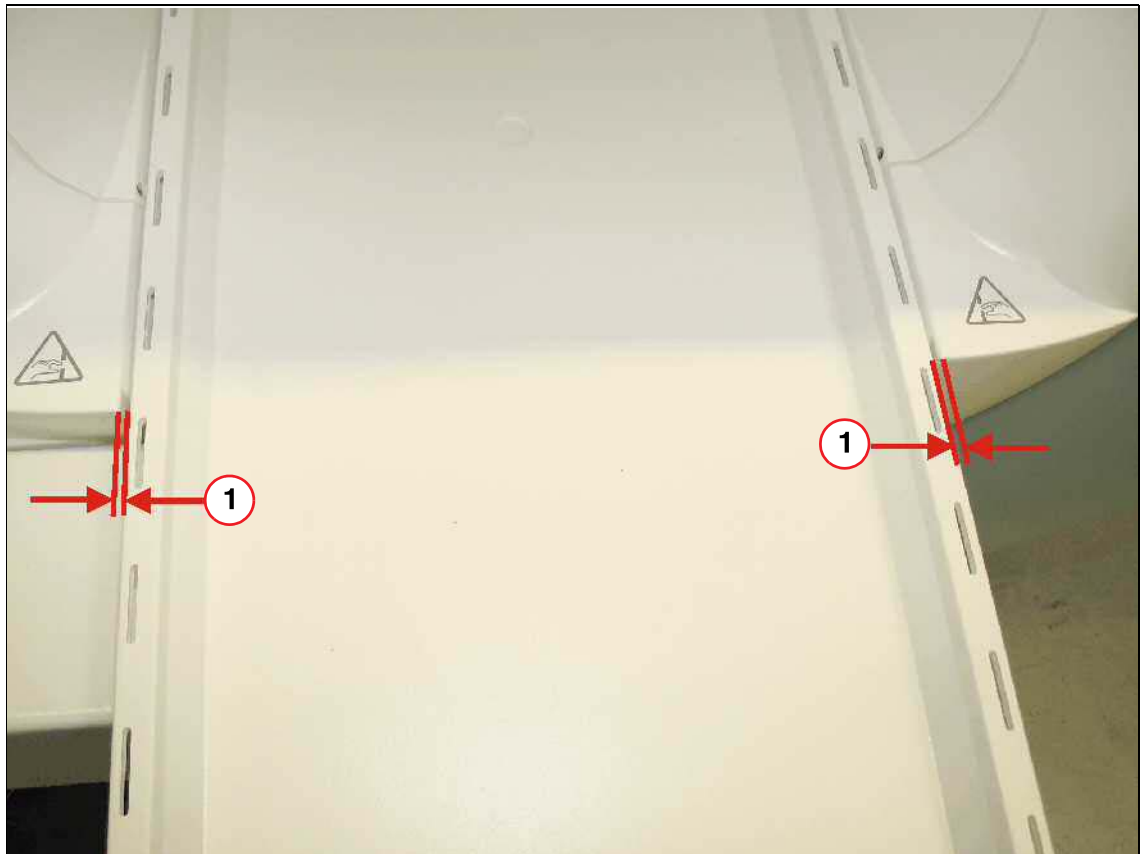
Fig. 443: Case 2: Checking the distance between patient table and cover / body coil (patient end) Pos. 1 Distance to be measured
