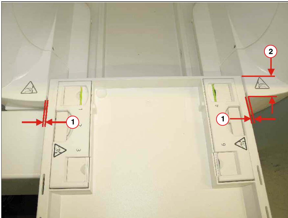
Fig. 442: Case 1: Checking the distance between patient table and cover (patient end)
