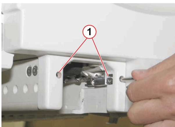
Fig. 537: Toothed belt tension adjustment Pos. 1 Adjustment screws for the belt tension
