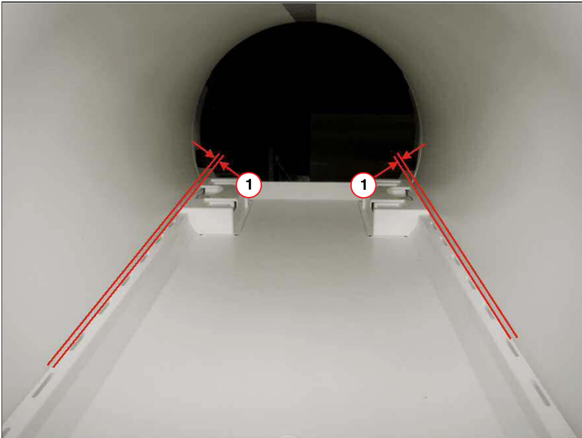
Fig. 444: Case 3: Checking the distance between patient table and Body Coil / cover (service end) Pos. 1 Distance to be measured
