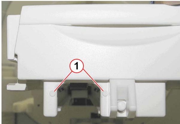
Fig. 535: Partial body patient table foot end side Pos. 1 Blanking plug
