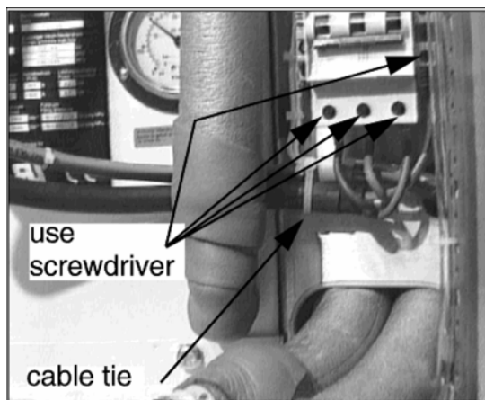
Fig. 499: Electrical disconnection of the cool pack
