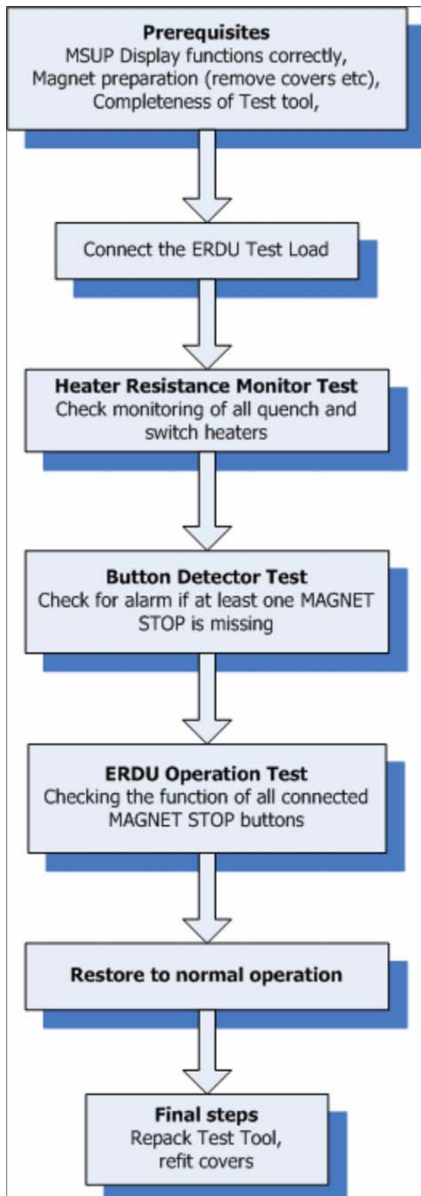
Fig. 455: ERDU testing flow chart
