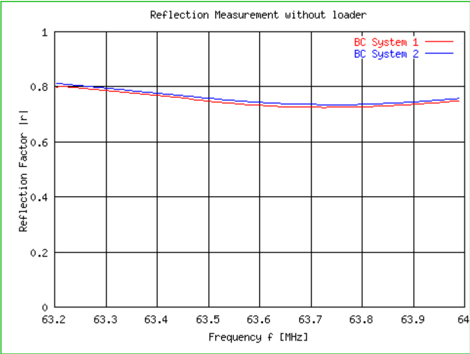
Fig. 369: BC - Reflection Evaluation
