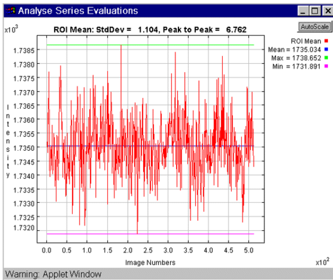
Fig. 146: ROI Mean (%) StdDev Peak to Peak Series Calculation
