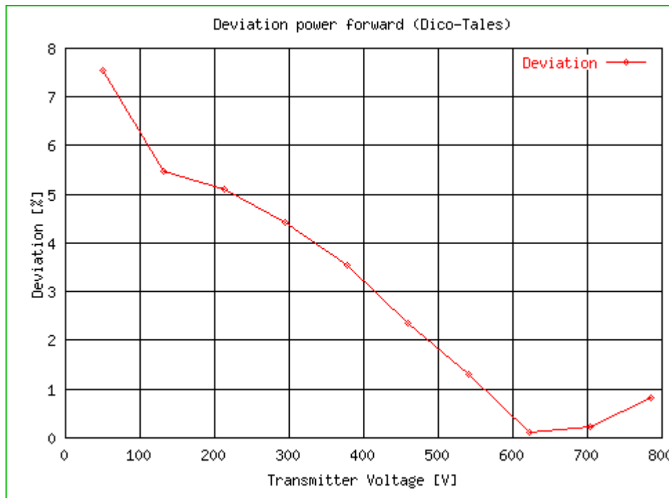
Fig. 362: Deviation between DICO and TALES
