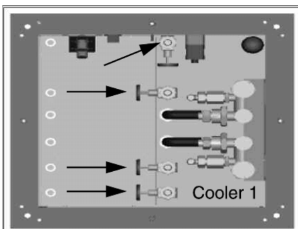
Fig. 493: Secondary valves
