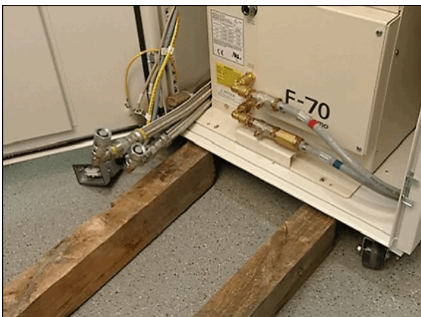
Fig. 518: Supporting ramp
