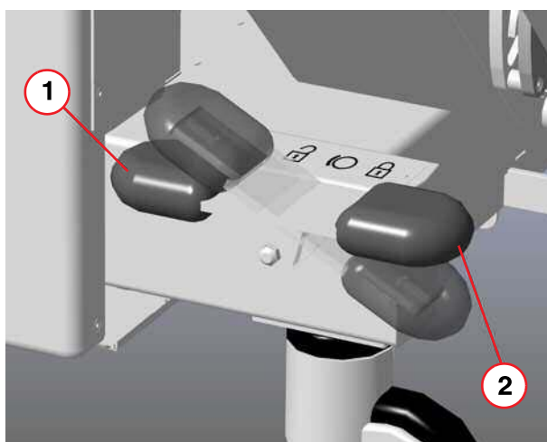
Fig. 445: Trolley brake, foot end
