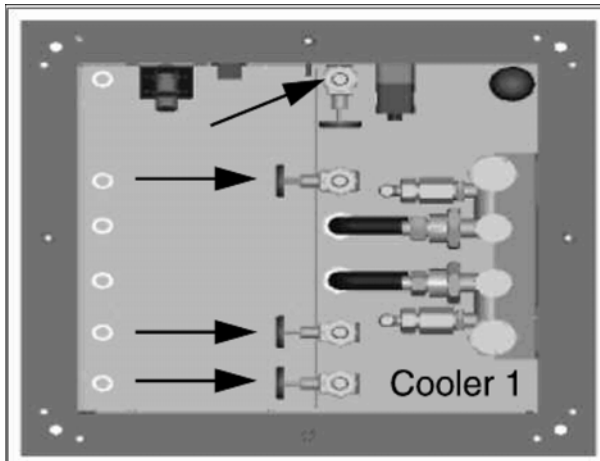
Fig. 484: Secondary valves
