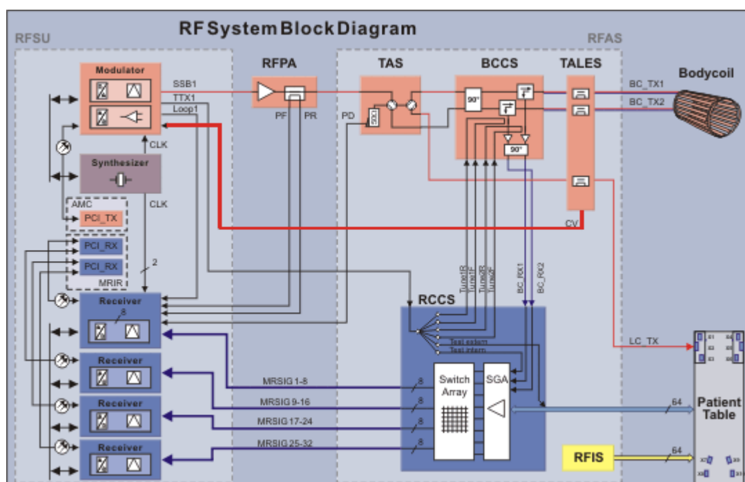
Fig. 363: Local Coil TX Path
