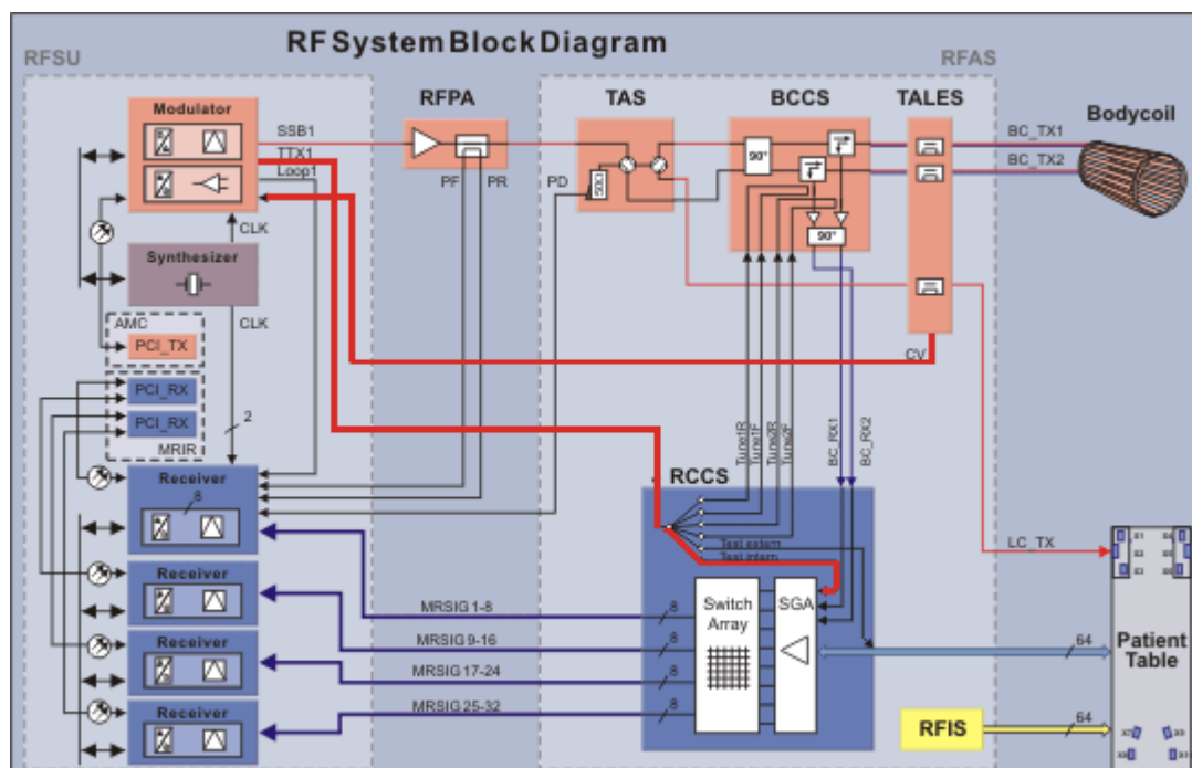
Fig. 349: RCCS SGA Loop (high gain)
