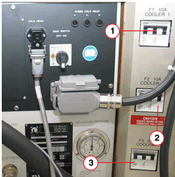
Fig. 513: RCA cabinet - Circuit Breakers F1, F2, F3
