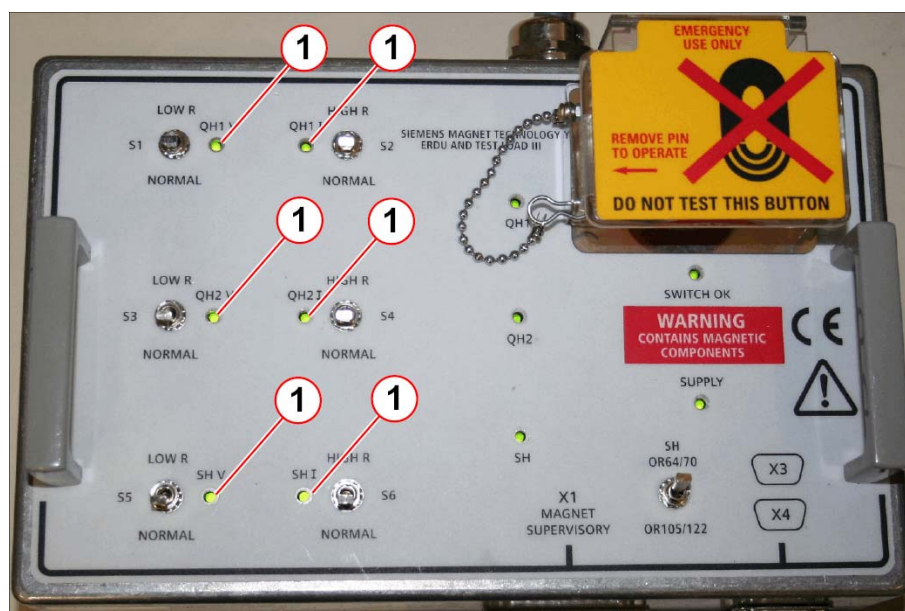
Fig. 461: ERDU Test load with ERDU pressed
