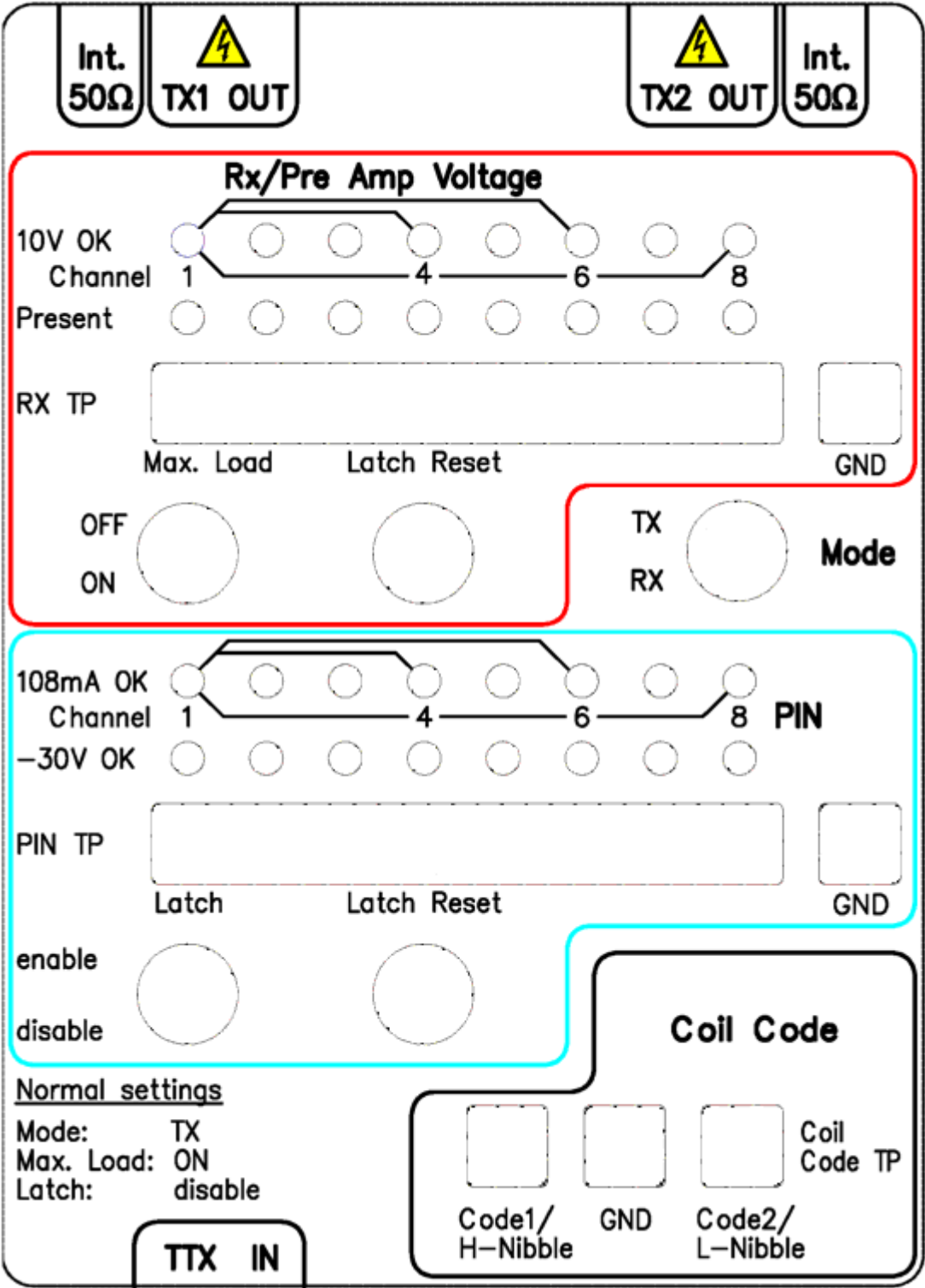
Fig. 328: Front Plate Service Plug
