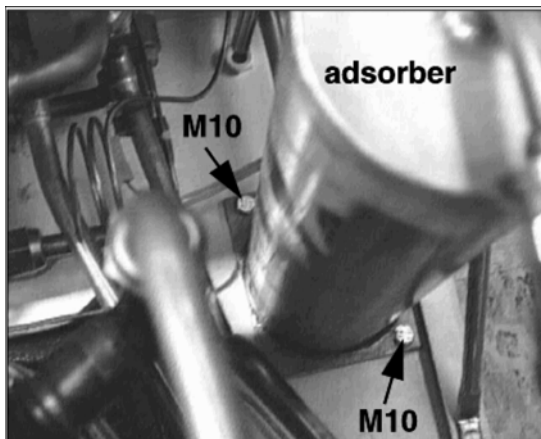
Fig. 503: Adsorber
