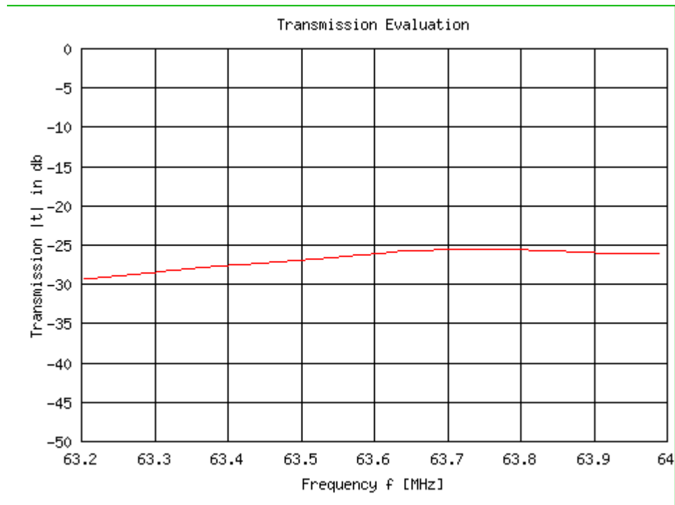
Fig. 367: BC - Transmission Evaluation
