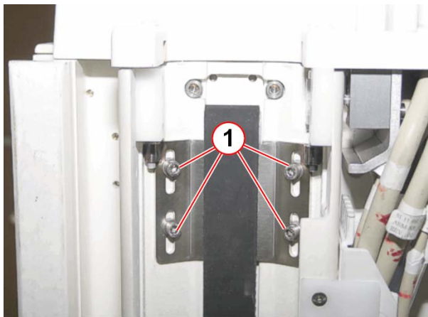
Fig. 536: Tension unit for the toothed belt Pos. 1 Fixing screws (4 mm Allen screw)
