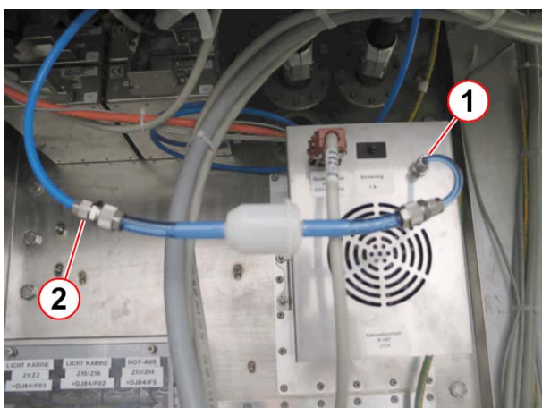
Fig. 541: External air filter of the vacuum pump
