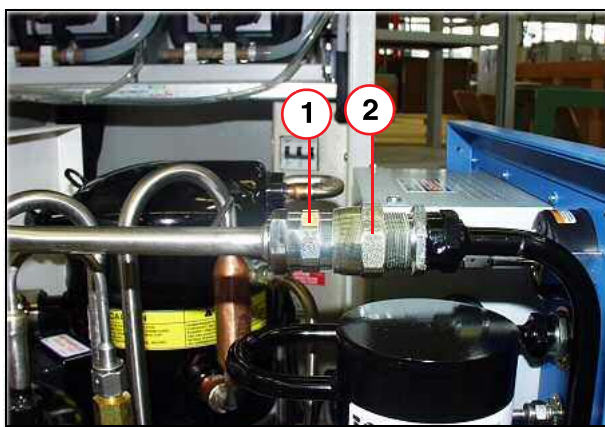
Fig. 510: Adsorber coupling
