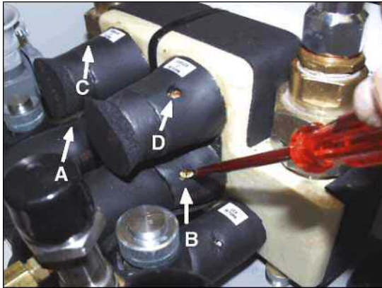
Fig. 479: Intake and outlet valves
