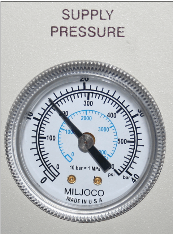
Fig. 527: F70 Static pressure reading
