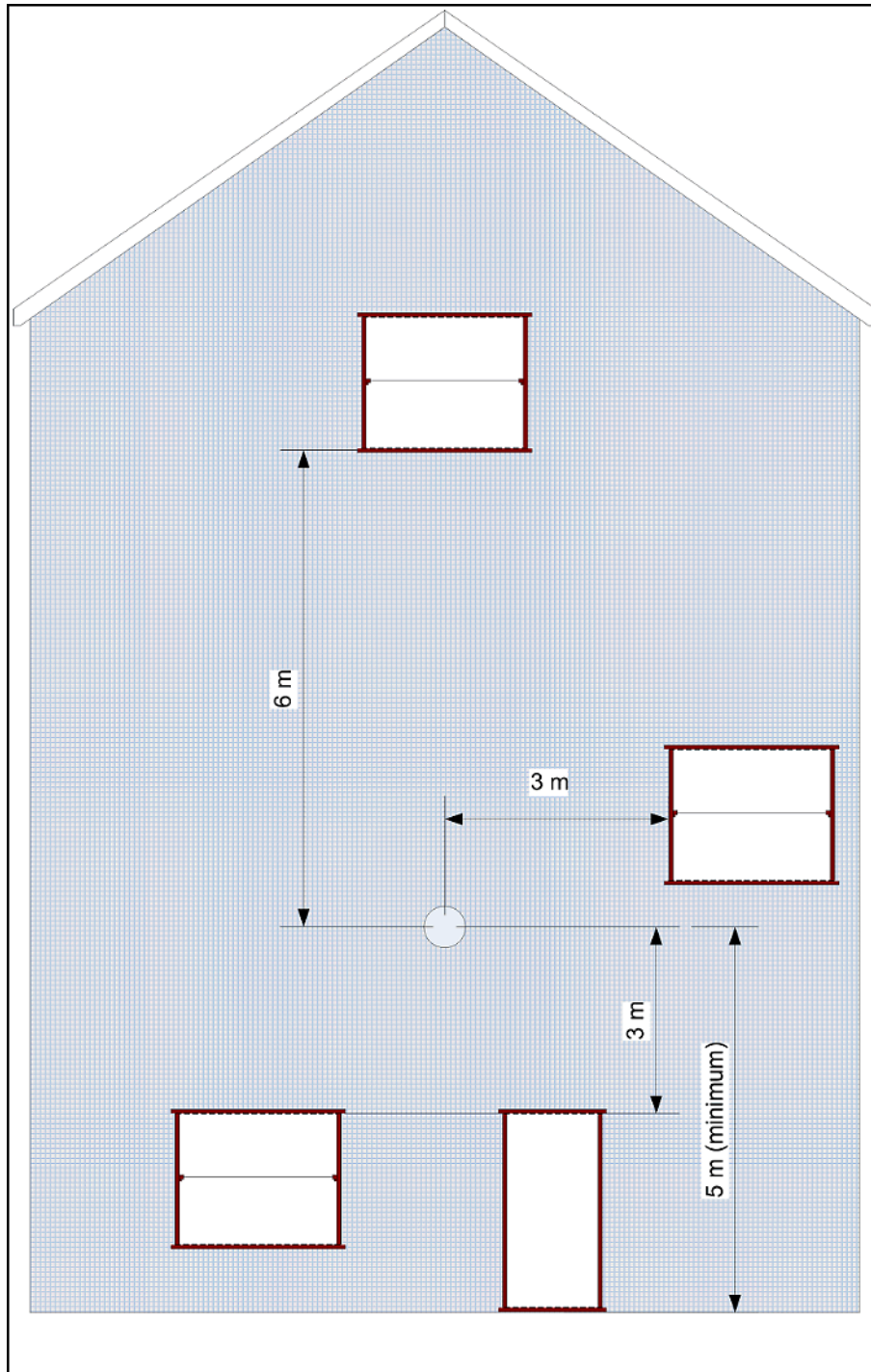
Fig. 409: Quench tube - example of venting to the outside
