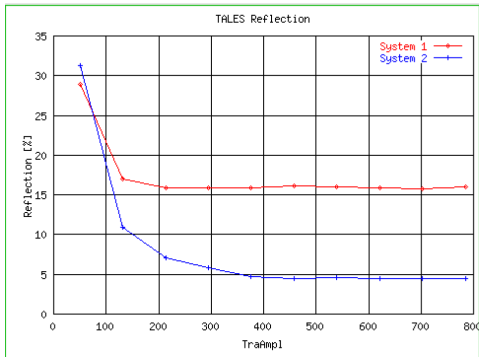
Fig. 368: BC power test - TALES reflection with load
