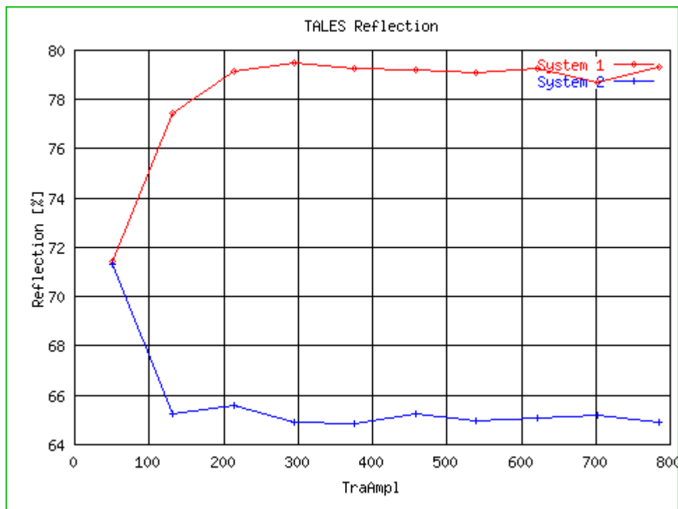
Fig. 371: TALES reflection without load
