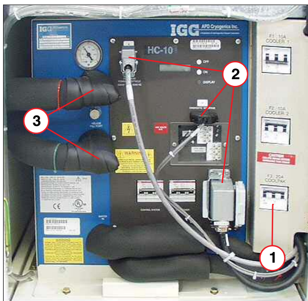
Fig. 504: Compressor
