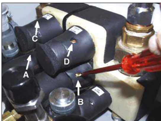
Fig. 488: Intake and outlet valves
