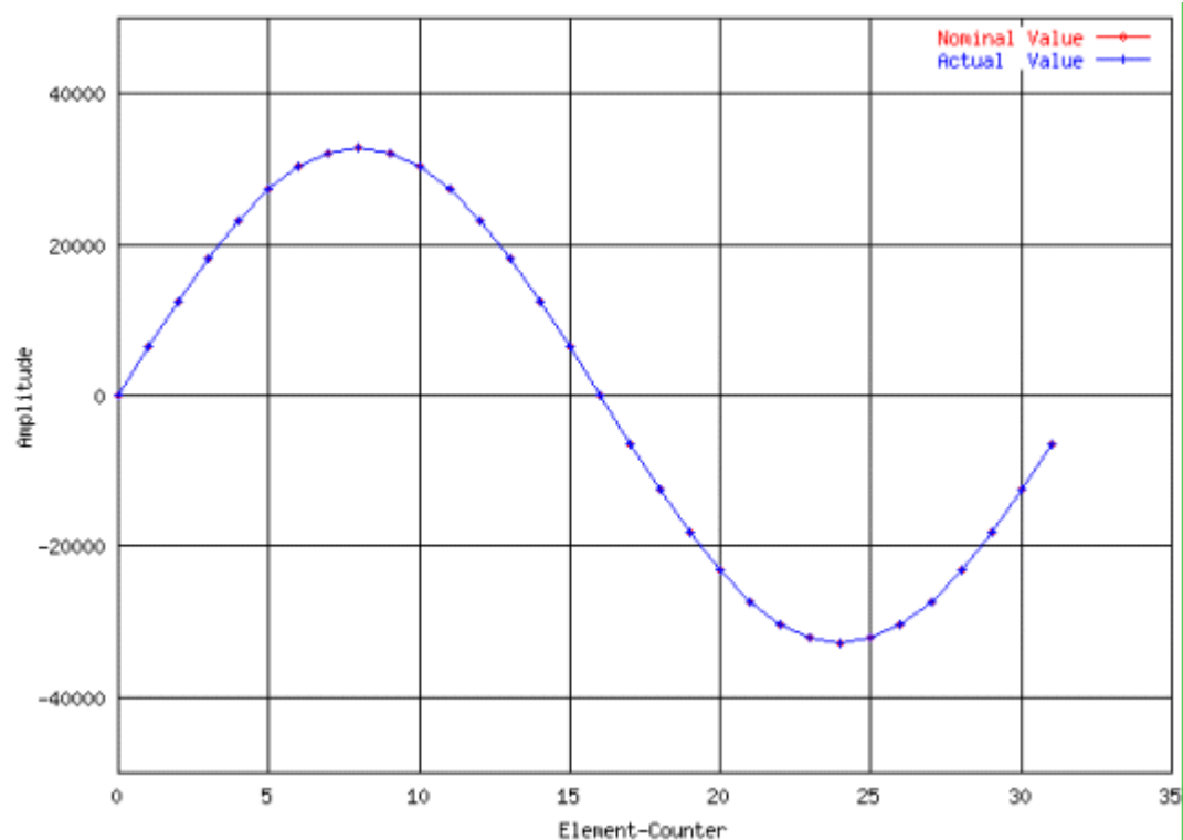
Fig. 329: Sine-shaped test pattern (TxTlkLocalLoop)
