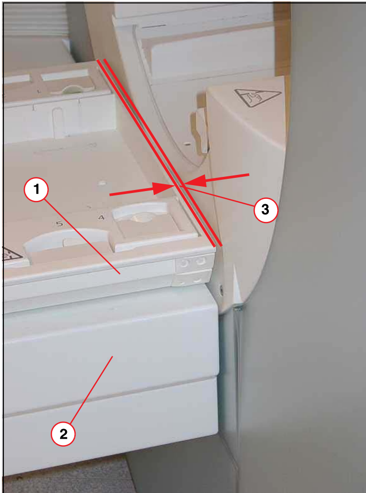
Fig. 441: Clearance, vertical gap
