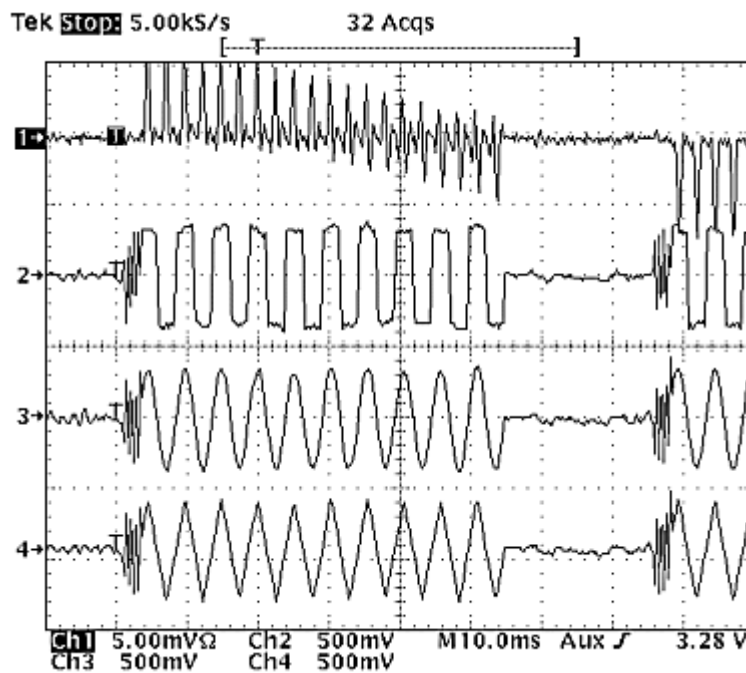
Fig. 334: Overview pulse diagram
