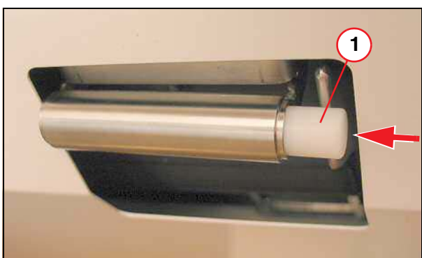
Fig. 436: Emergency release Pos. 1 Release button
