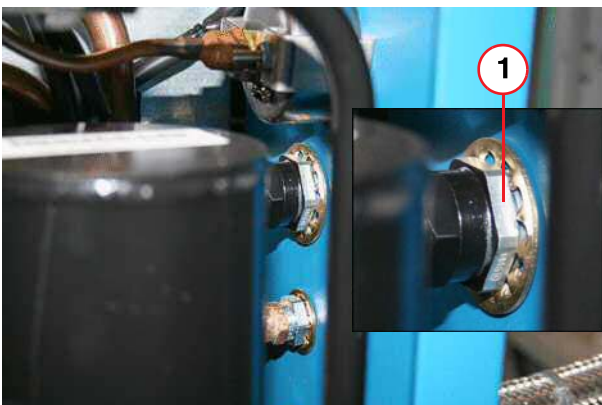
Fig. 522: F70 Adsorber - high pressure supply coupling (inlet side) Pos. 1 HOLD stationary nut ( 1" open-end spanner/wrench)
