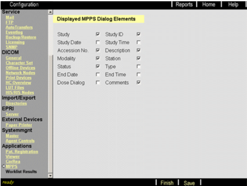
Fig. 62: Modality Performed Procedure Steps
