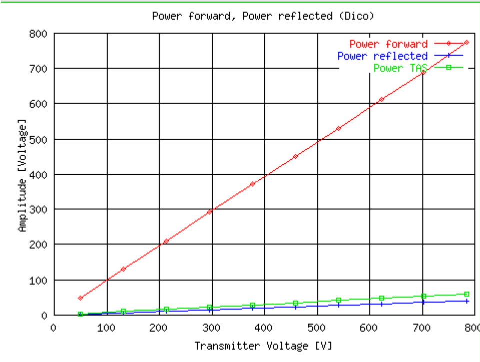
Fig. 358: Power forward, reflected (DICO): Power reflected TAS_3TM Example Output
